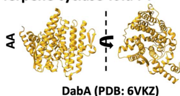
Fig. 2 AA and peptide PT structural folds, and the reactions catalysed by PTs. Experimentally determined ABBA-fold PTs (purple) include representatives from the DMATS (CymD, AuraA), and cyanobactin PT family (PagF). IDS-like PTs (blue) are predicted structures from ref. 10 (AgdS) and ref. 23 (PalQ), while a single experimentally determined structure was obtained from the terpene cyclase-like PTs (yellow, DabA).
