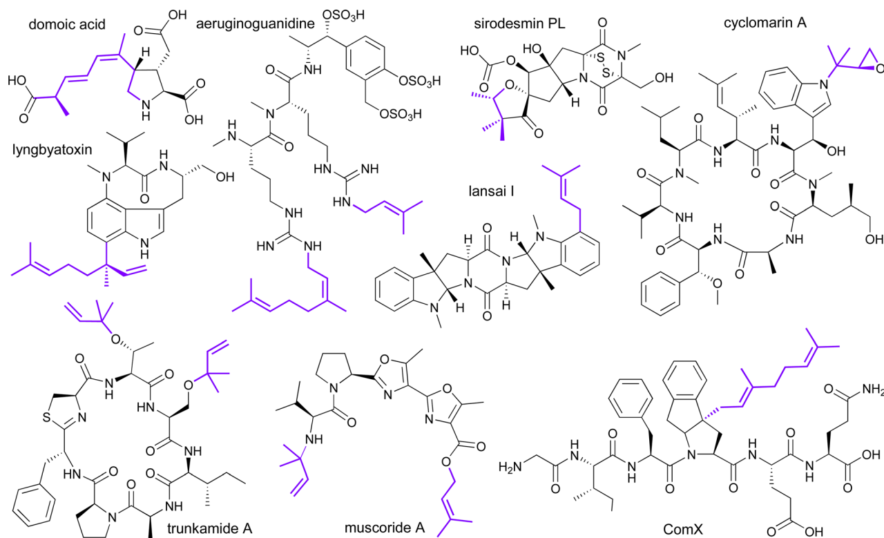
Fig. 1 Prenylated bioactive NPs: domoic acid (monomer AA; Glu forward N -geranylation), aeruginoguanidine A (NRP; Arg forward N -pre-nylation/-geranylation), sirodesmin PL (alkaloid; Tyr forward O -pre-nylation), cyclomarin A (NRP; Trp reverse N -pre-nylation), lyngbyatoxin A (NRP; dipeptide reverse C -geranylation), lansai I (DKP; dipeptide reverse C -pre-nylation), trunkamide A (RiPP; peptide reverse O -pre-nylation), muscoride A (RiPP; reverse N -terminal and forward C -terminal prenylation) and ComX (RiPP; peptide forward C -geranylation).
