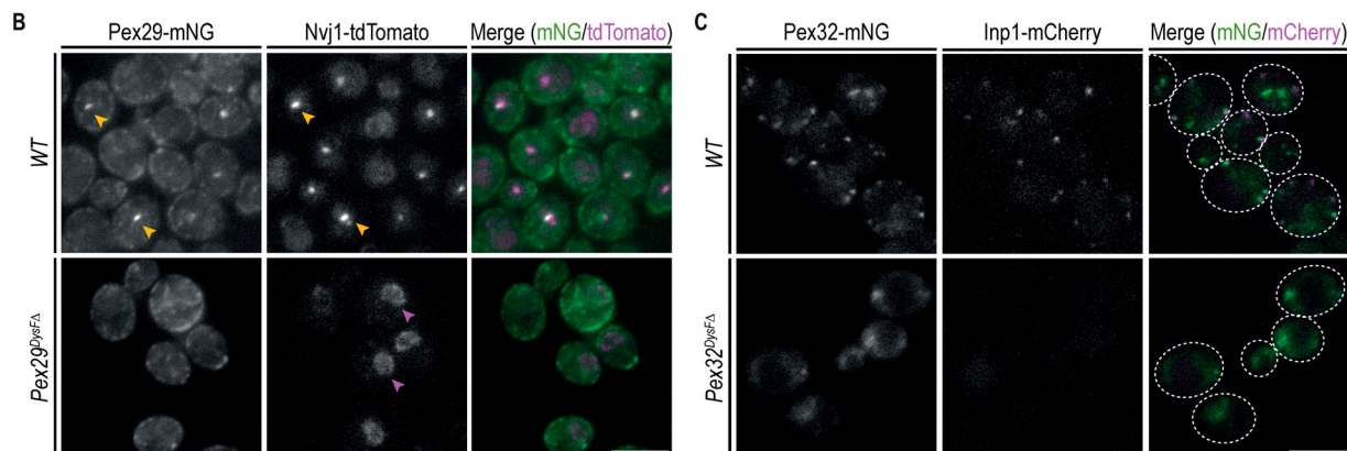
Figure S2. DysF domains of Pex30 adaptors are also required for complex localization. (A) Crude membrane fractions of cells expressing endogenously tagged variants of Pex28-13xMyc, Pex29-V5, and Pex32-3xHA, or untagged proteins as control, were solubilized with detergent, and the extracts were subjected to immunoprecipitation (IP) with anti-Myc, V5, or HA antibodies. Eluted proteins were separated by SDS-PAGE and analyzed by western blotting. Pex28-Myc, Pex29-V5, Pex30, and Pex32-HA were detected with anti-Myc, anti-V5, anti-Pex30, and anti-HA, respectively. Dpm1, used as a loading control, was detected with anti-Dpm1 antibody. *, IgG light chain. IB, immunoblot. The position of molecular weight markers (in kDa) is indicated. (B) Localization of endogenous Pex29-mNG variants and Nvj1-tdTomato in cells during the diauxic shift. Yellow arrowheads highlight colocalization between Pex29 and Nvj1, and magenta arrowheads highlight the non-concentrated Nvj1. Bar, 5 μm. (C) Localization of endogenous Pex32-mNG variants and Inp1-mCherry in exponentially growing cells. Bar, 5 μm. Source data are available for this figure: SourceData FS2.
