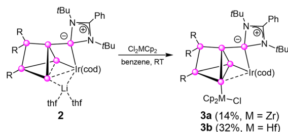
Scheme 2 Synthesis of group 4 metallocenyl-substituted iridasiliconoids 3a,b from 2 and Cl 2 MCp 2 (M = Zr ( 3a ), Hf ( 3b ); ● = Si; R = 2,4,6-triisopropylphenyl; cod = 1,5-cyclooctadiene).
