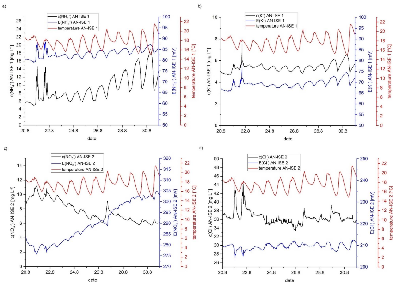
Fig. 2 Temperature dependent fluctuations in the mV signals and concentration readings of (a) NH_4^+ (AN-ISE 1), (b) K^+ (AN-ISE 1), (c) NO_3^- (AN-ISE 2), (d) Cl^- (AN-ISE 2); Bickenalb River, 20.–30.08.2022.
