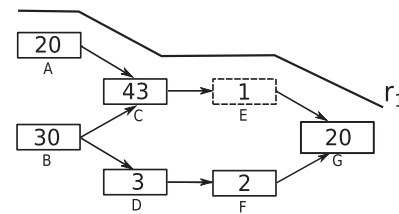
Fig. 1. A toy DBG with one traversing read shown denoted r_1 . Nodes in the DBG represent k -mers, numbers inside nodes represent the abundance of the corresponding k -mer in the data. Dashed node represents the k -mer, which will be lost if r_1 is removed
