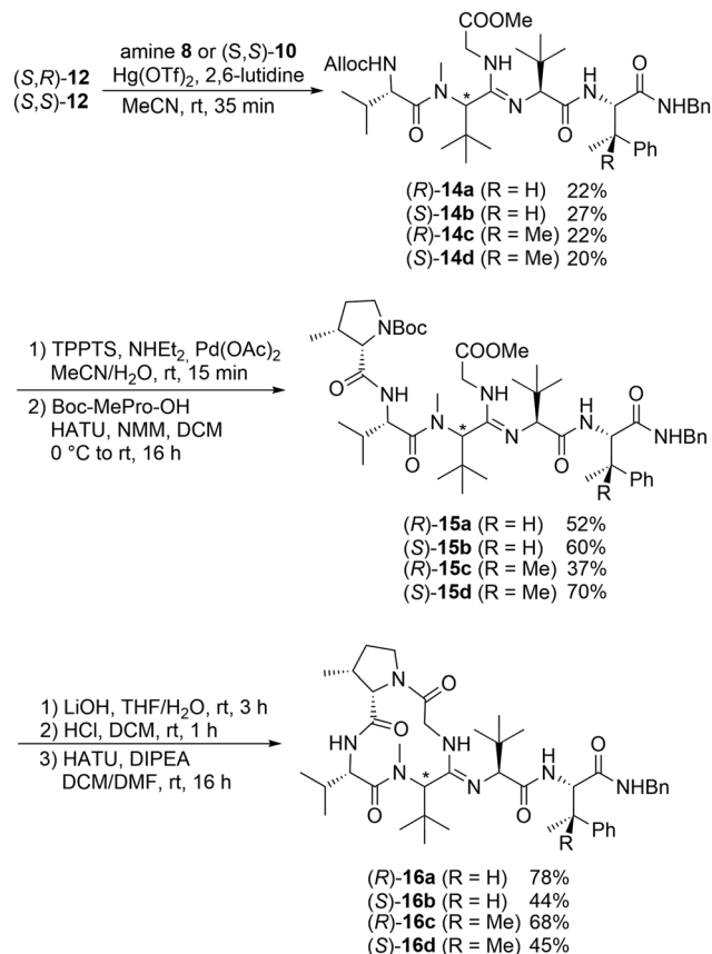
Scheme 4 Synthesis of bottromycin derivatives 16 . Abbreviation: TPPTS: tris(trimethylsilyl)phosphine.
