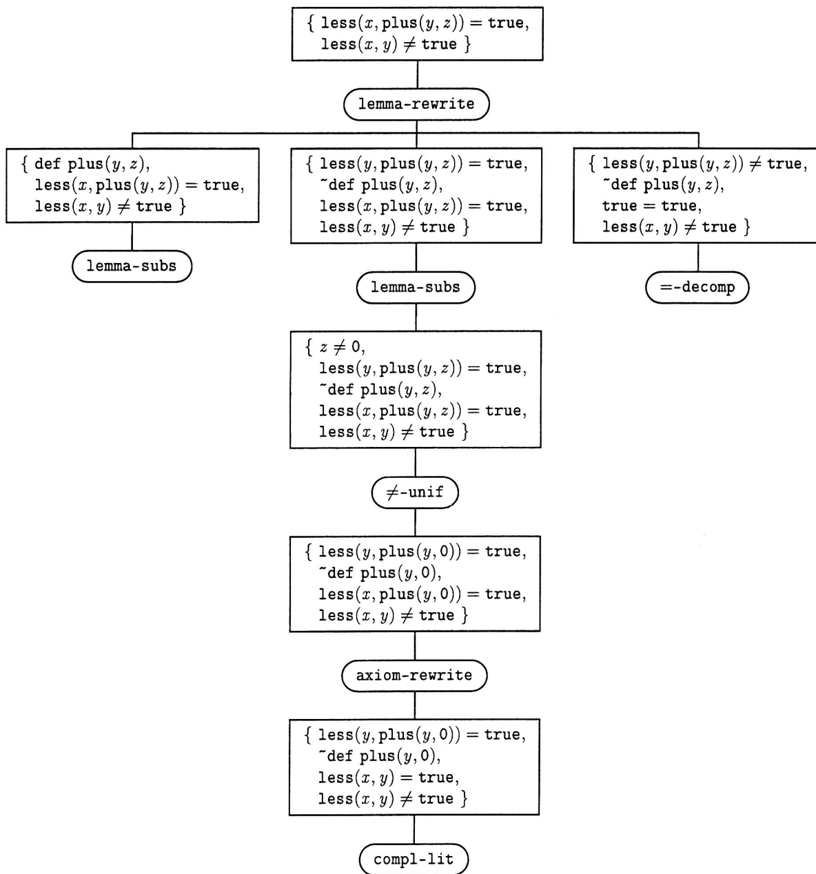
Figure 1: Proof State Tree for Example 3.1
