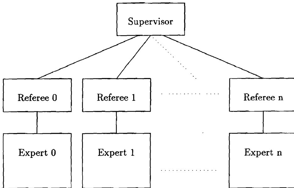
Figure 1: Basic structure of a team in the TEAMWORK method
