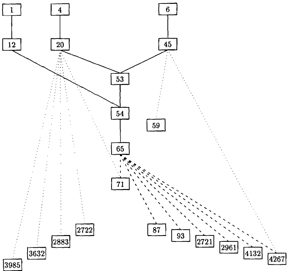
Figure 3: Proof graph corresponding to the example on page 30
