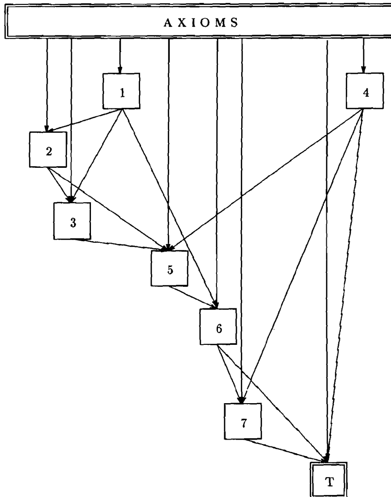
Figure 7: Lemma structure according to B.1.3
