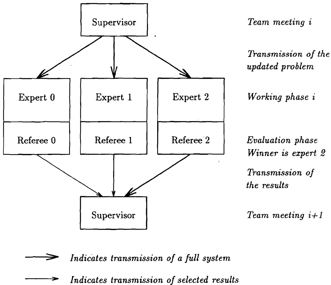
Figure 2: A cycle between two team meetings
