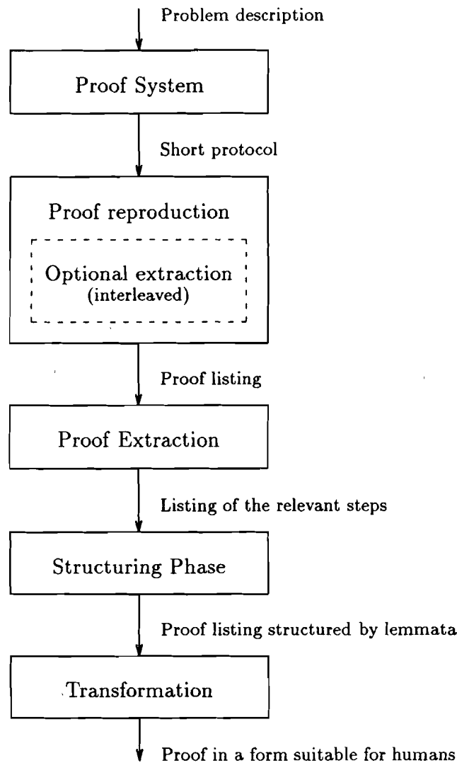
Figure 6: Structure of the implemented system
