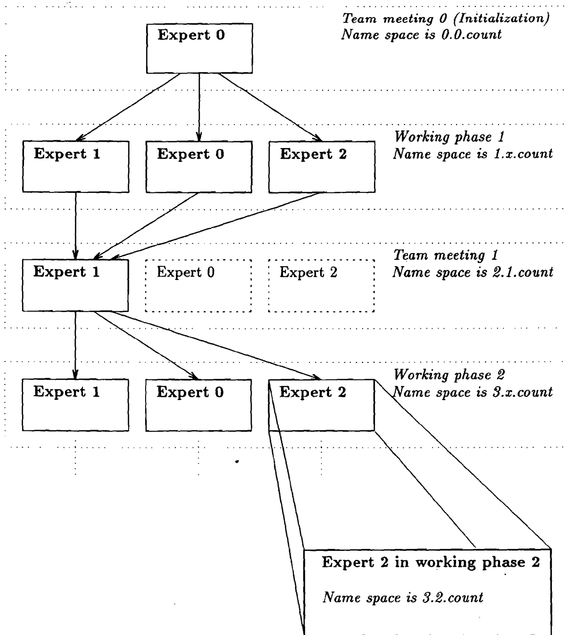
Figure 4: Team work and name spaces
