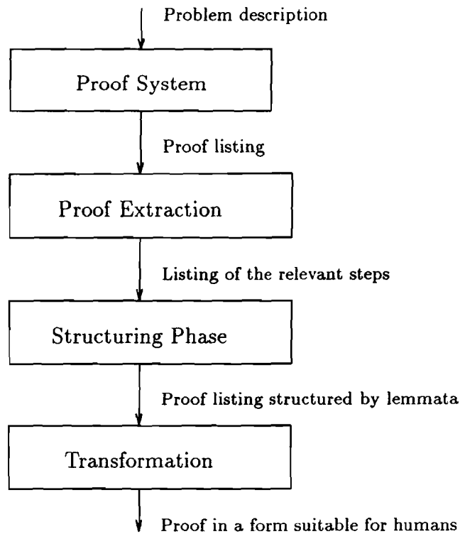
Figure 5: A concept for a system generating, analyzing and transforming proofs
