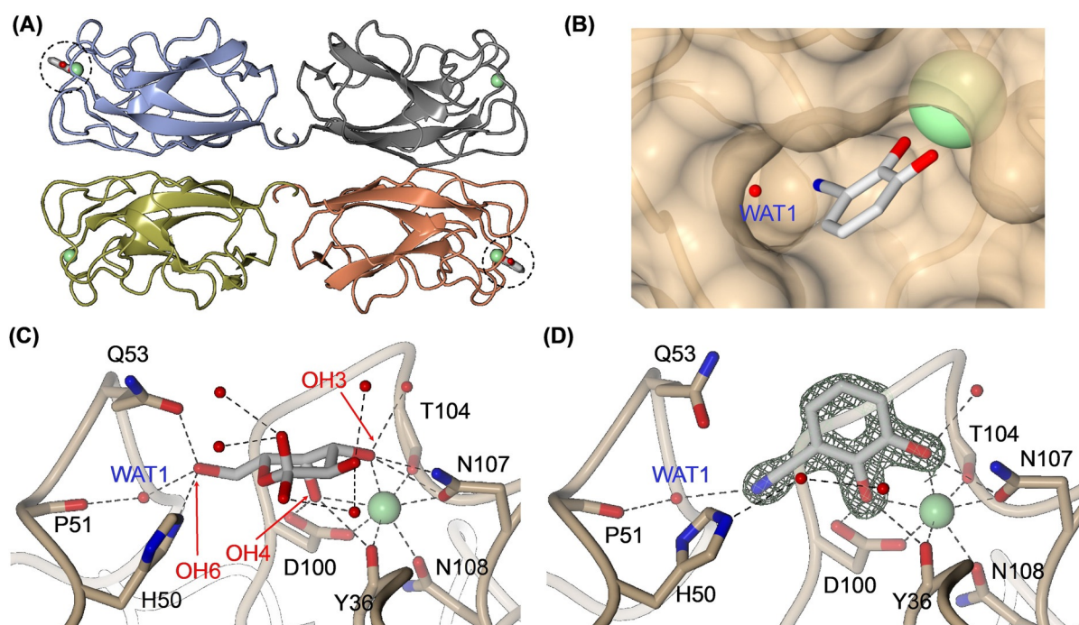
Figure 5. A) Overall structure of LecA-3 complex (PDB code: 6YO3). 2 molecules of compound 3 are shown as sticks and the \text{Ca}^{2+} ions as green spheres. Dotted circles indicate the binding sites of 3 . Each LecA monomer is depicted as cartoon in different colors. B) Surface display of compound 3 at the binding site. C) Interaction of galactose with LecA (PDB code: 1OKO). D) Interaction of 3 with LecA, electron density is displayed at 1\sigma .
