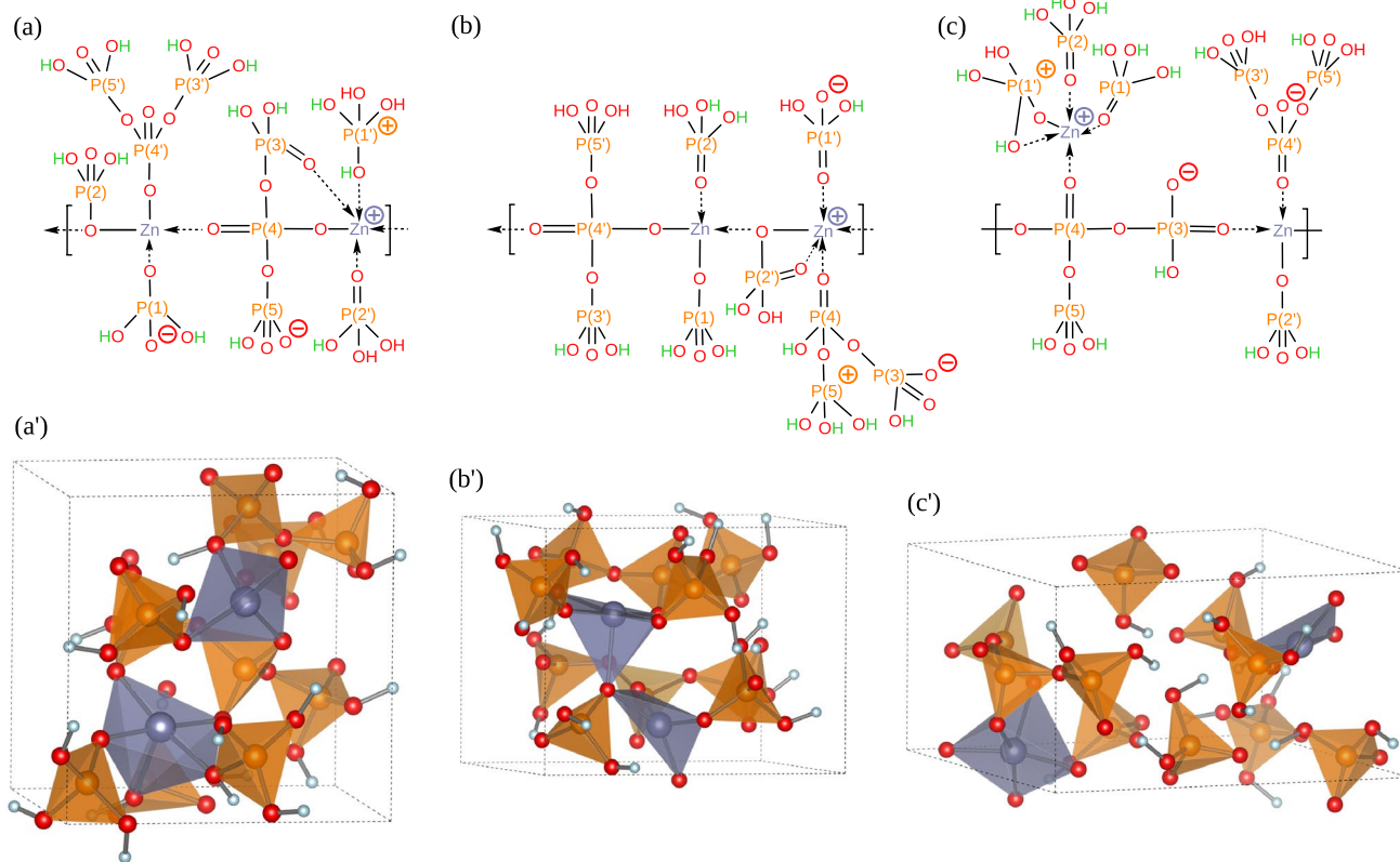
Fig. 2 Lewis (a–c) and three-dimensional (a'–c') structures of the system after decompression from a isotropic, b uniaxial, and c volume-conserving compressions. Dashed arrows indicate ionic bonds. Zinc, phosphorus and oxygen are presented in gray, orange and red colors, respectively. Formal positive charges are always assigned
