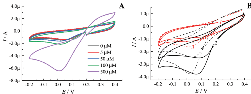
Fig. 4 CV responses of the Pd-NPs-modified GCE recorded at a scan rate 50 \text{ mV s}^{-1} in phosphate buffer (A) with various \text{H}_2\text{O}_2 concentration at pH 7.5 (the experiments were performed under an inert atmosphere) and in 50 \mu\text{M H}_2\text{O}_2 (B) at different pH values: pH 7.5 (1 and 2) and pH 5.5 (3 and 4) under (1 and 3) inert and (2 and 4) air atmospheres.
