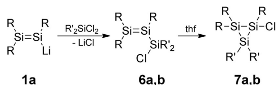
Scheme 3. Synthesis of \alpha -chlorosilyldisilenes 6 a,b and cyclotrisilanes 7 a,b ( R = \text{Tip} ; 6 a , 7 a : R' = \text{Me} ; 6 b , 7 b : R' = \text{Ph} ). [12]
