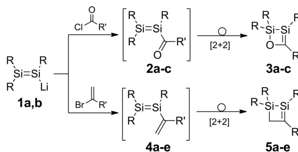
Scheme 2. Synthesis of cyclic silenes 3 a–c and 5 a–e ( 1 a : R = Tip = 2,4,6- i Pr 3 C 6 H 2 ; 1 b : R = SiMe 2 Et; 2 a , 3 a : R = Tip, R' = t Bu; 2 b , 3 b : R = Tip, R' = 1-adamantyl; 2 c , 3 c : R = SiMe 2 Et, R' = 1-adamantyl; 4 a , 5 a : R = Tip, R' = Ph; 4 b , 5 b : R = Tip, R' = SiMe 3 ; 4 c , 5 c : R = SiMe 2 Et, R' = H; 4 d , 5 d : R = SiMe 2 Et, R' = Ph; 4 e , 5 e : R = SiMe 2 Et, R' = SiMe 3 ). [8,9]
