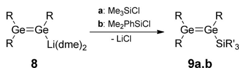
Scheme 4. Previously reported synthesis of unsymmetrically substituted digermenes 9 a,b ( R = \text{Tip} = 2,4,6\text{-}i\text{Pr}_3\text{C}_6\text{H}_2 ; 9 a : \text{SiR}'_3 = \text{SiMe}_3 ; 9 b : \text{SiR}'_3 = \text{SiMe}_2\text{Ph} ). [13]
