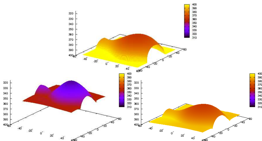
Figure 3: The Phong-surface vase experiment, colour-coded depth maps. Top: Exact solution. Bottom left: Lambertian reconstruction. Bottom right: VBW/P reconstruction.
