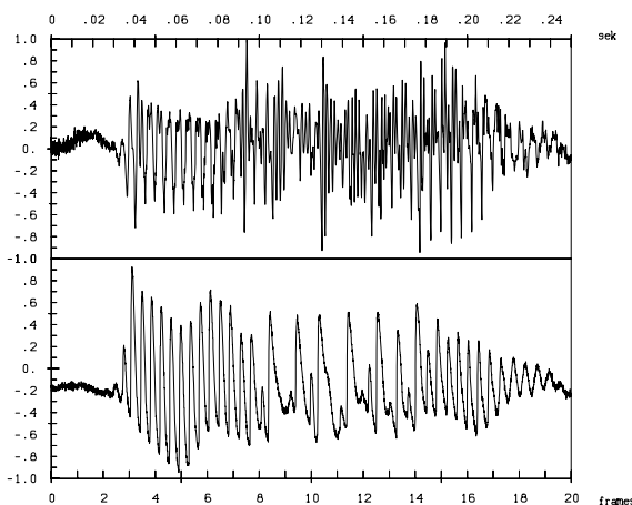
Figure 1: Top: Speech signal with laryngealization. Bottom: Voice source signal, recorded with a laryngograph.
