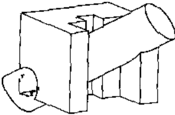
Addition A \cup B
