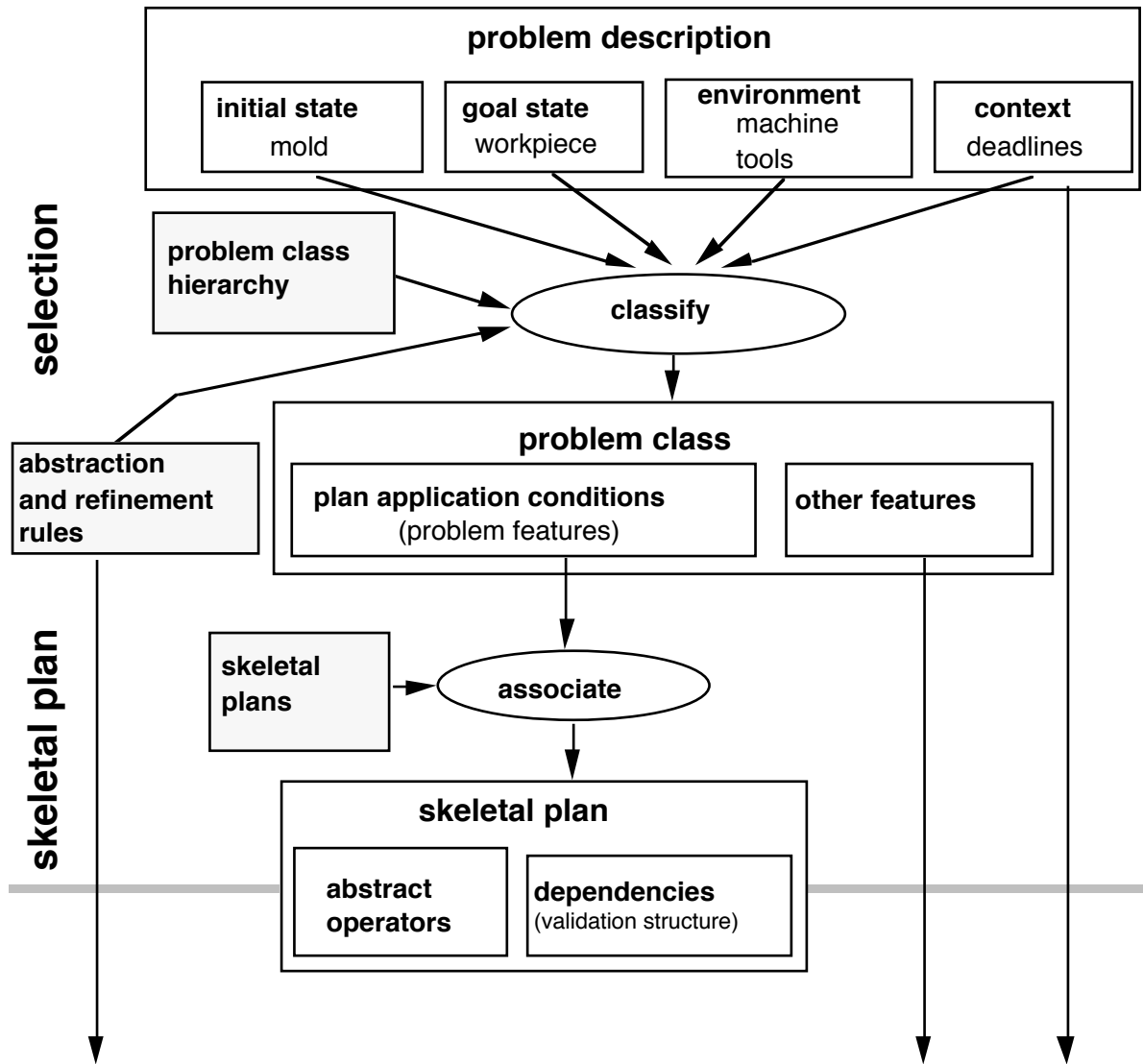
Figure 3a: Detailed inference structure for skeletal plan selection, the first subtask in hierarchical skeletal plan refinement
