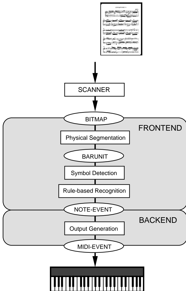
Fig.3: The DOREMIDI-System
