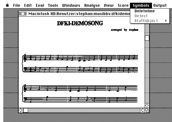
Fig.16: Staff removal
