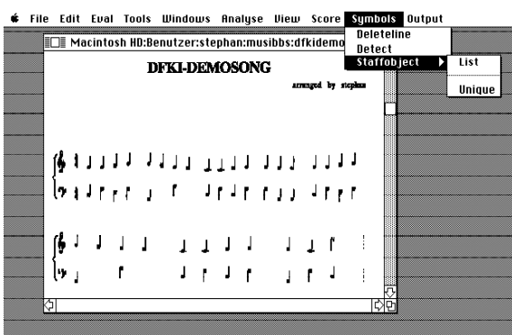
Fig.17: Symbolrecognition
