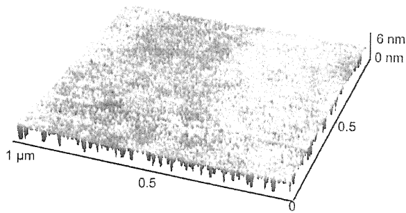
Fig. 5. AFM-photography of three layers AR-coating on glass after stack firing at 450°C for 15 min.
