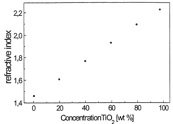
Fig. 1. Calculated refractive index (ellipsometry and reflection spectroscopy) at 550 nm of \text{SiO}_2/\text{TiO}_2 -layers on glass after thermal densification at 450°C, for 15 min. 0% \text{TiO}_2 corresponds to a pure \text{SiO}_2 -layer. The refractive index reproducibility of ten samples was \pm 1.5 \times 10^{-3} .
